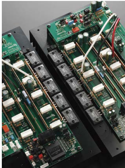
Dedicated Power Supply Components for V Amp Stage
