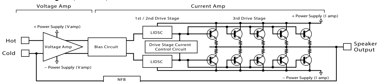
Grandioso S1 Block Diagram (1 Channel)
