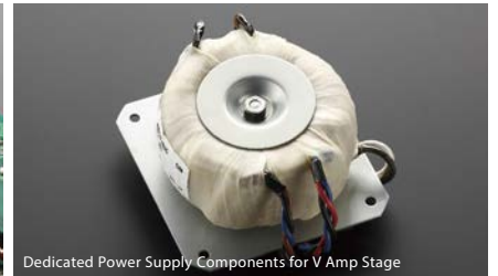
Dedicated Power Supply Components for V Amp Stage
