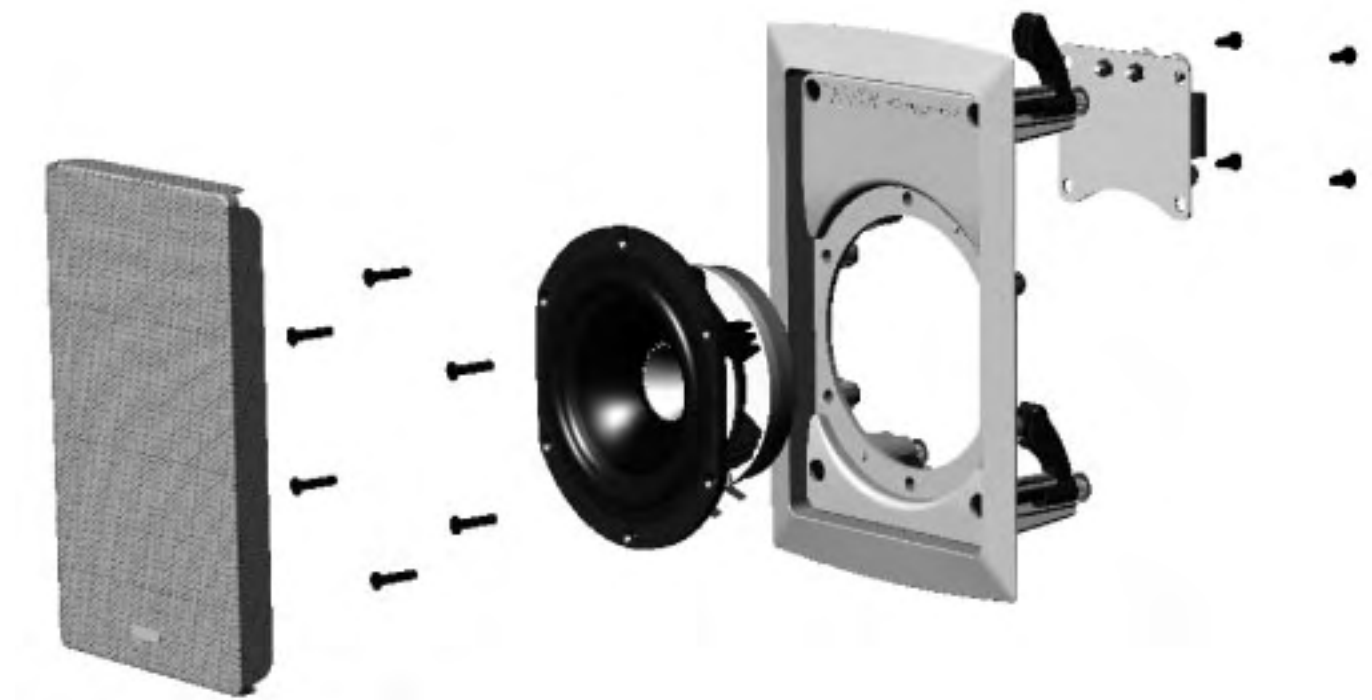
EXPLODED VIEW OF iw4DC
